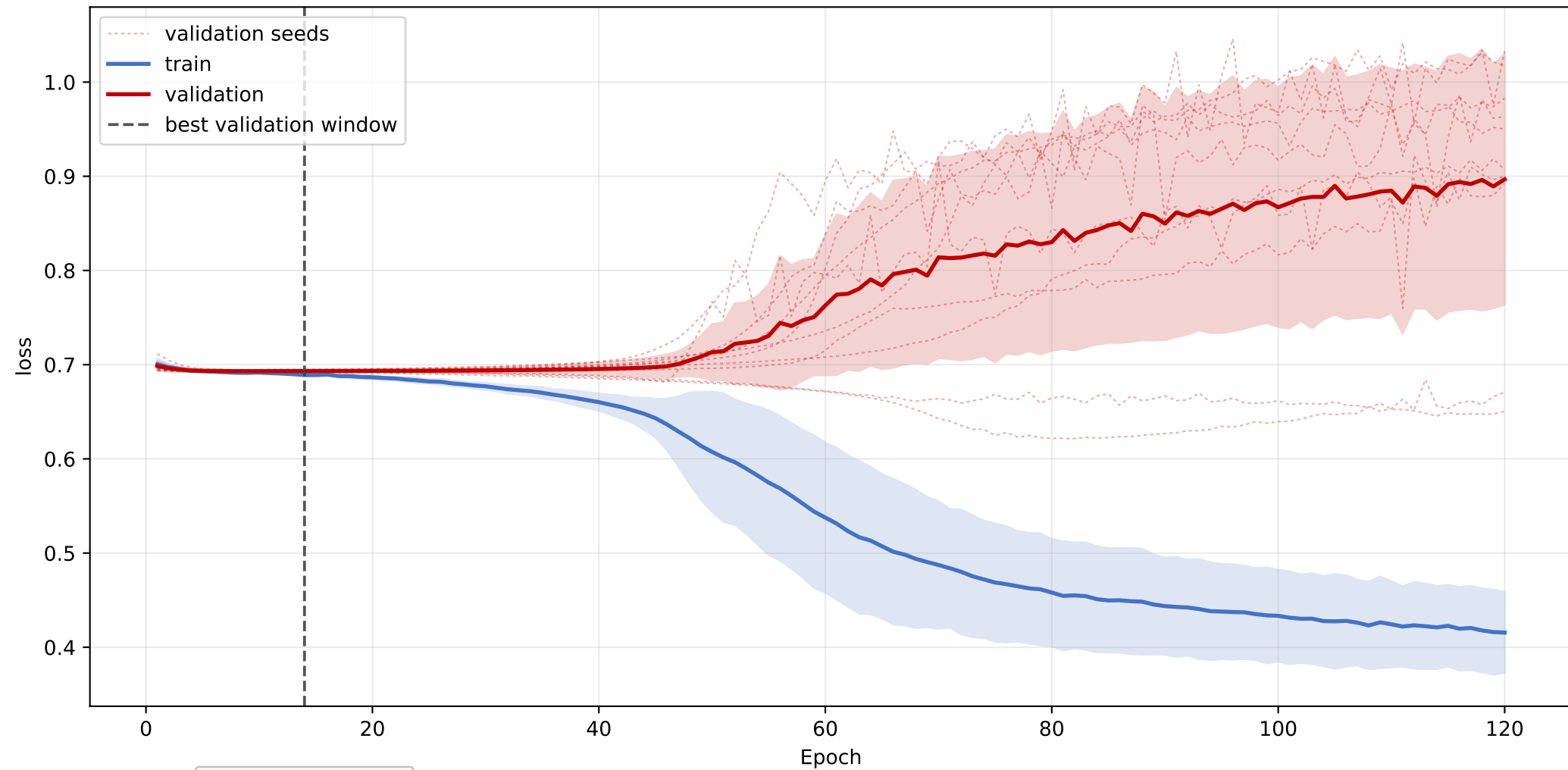
CerP+Hex2Cer+SHexCer_groups_glt: mean loss learning curve across seeds
