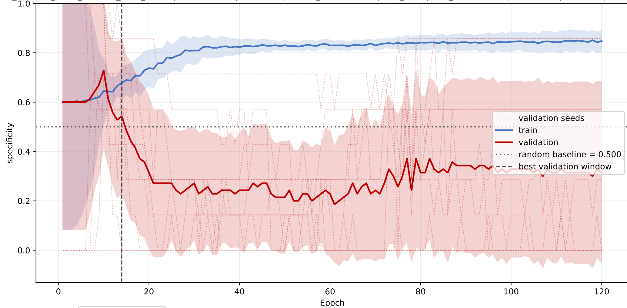
CerP+Hex2Cer+SHexCer_groups_gltf: mean specificity learning curve across seeds
