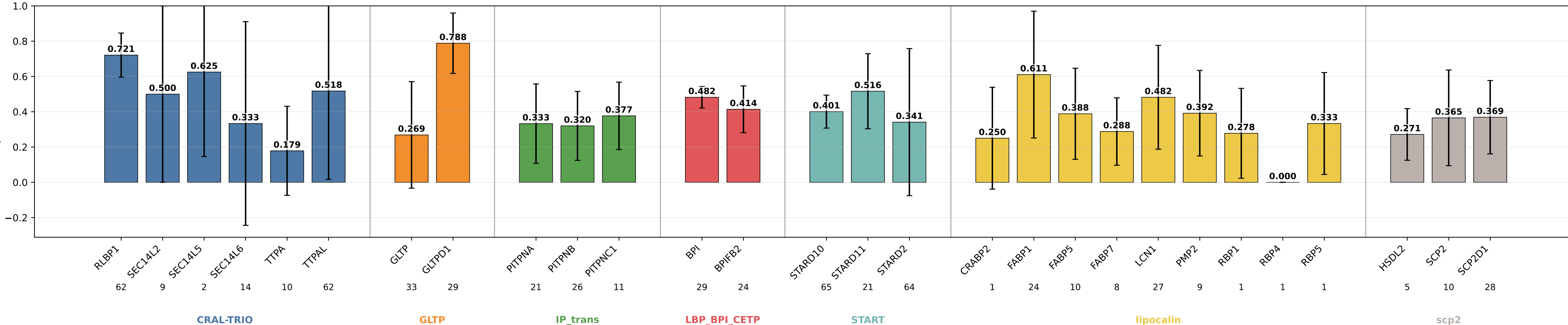
descriptors_pair_clean precision by subgroup descriptors_pair_clean | class weights | lr=0.0001 | weight_decay=0.01 | final_m=4 | final_dropout=0.1 | hiddim=8 | heads=8 | batch=16 | ep=120 | seeds=0,1,2,3,4
