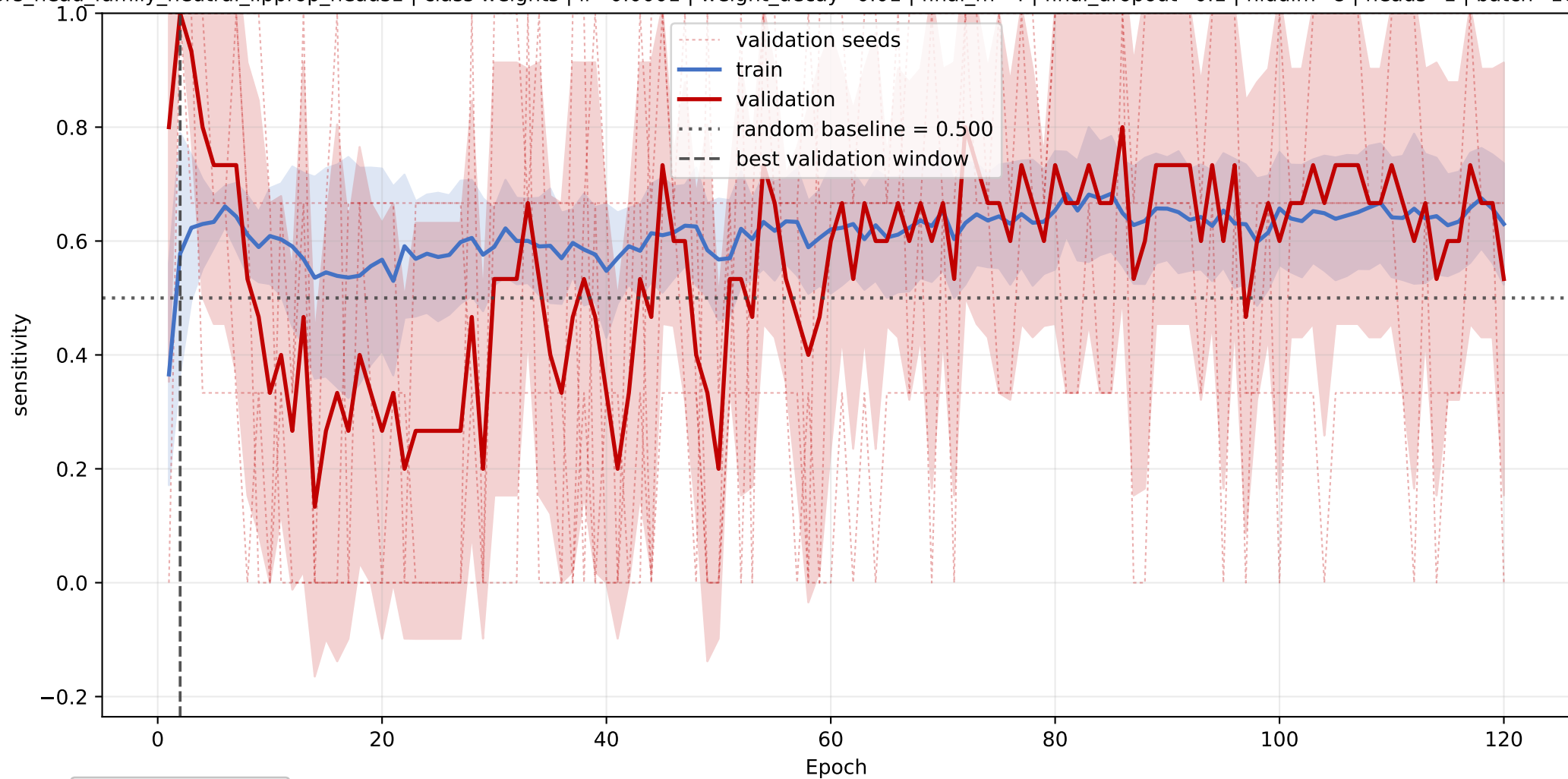
OSBP: mean sensitivity learning curve across seeds
