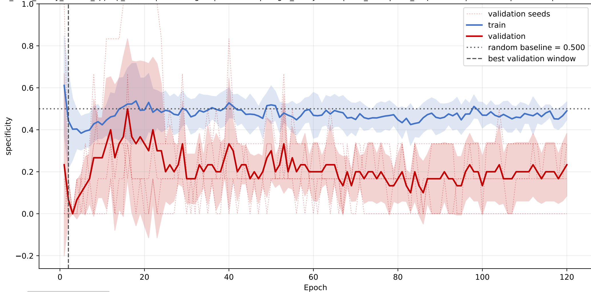
OSBP: mean specificity learning curve across seeds
