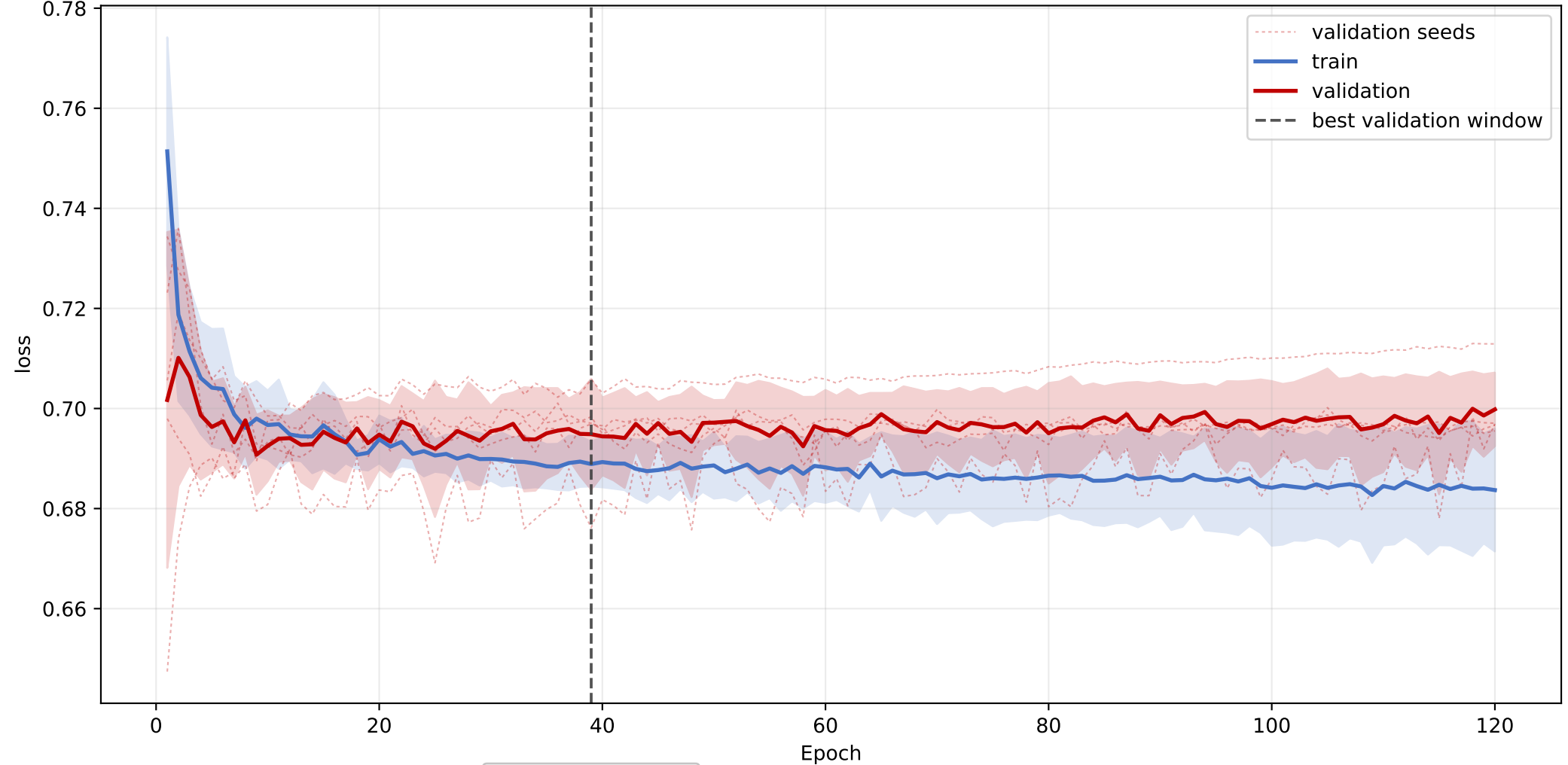
scp2: mean loss learning curve across seeds
