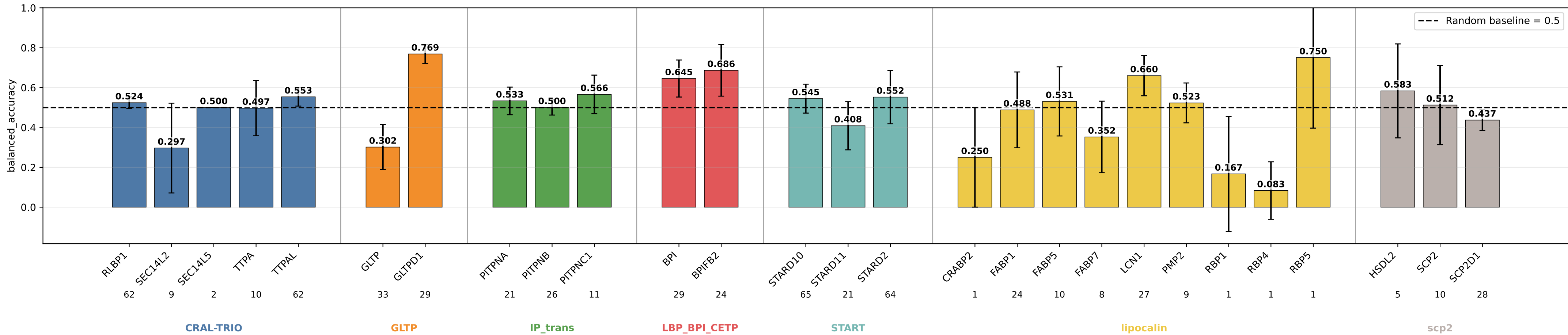
descriptors_head_family_neutral_lipprop_lambdasqrt balanced_accuracy by subgroup descriptors_head_family_neutral_lipprop_lambdasqrt | class weights | lr=0.0001 | weight_decay=0.01 | final_m=4 | final_dropout=0.1 | hiddim=8 | heads=8 | batch=16 | ep=120 | seeds=0,1,2,3,4
