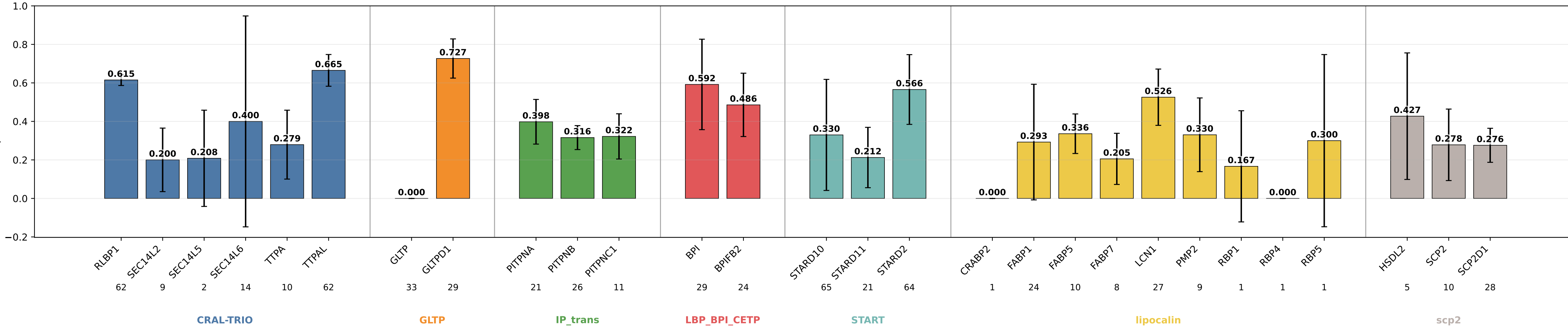
descriptors_head_family_neutral_lipprop_lambdasqrt precision by subgroup descriptors_head_family_neutral_lipprop_lambdasqrt | class weights | lr=0.0001 | weight_decay=0.01 | final_m=4 | final_dropout=0.1 | hiddim=8 | heads=8 | batch=16 | ep=120 | seeds=0,1,2,3,4
