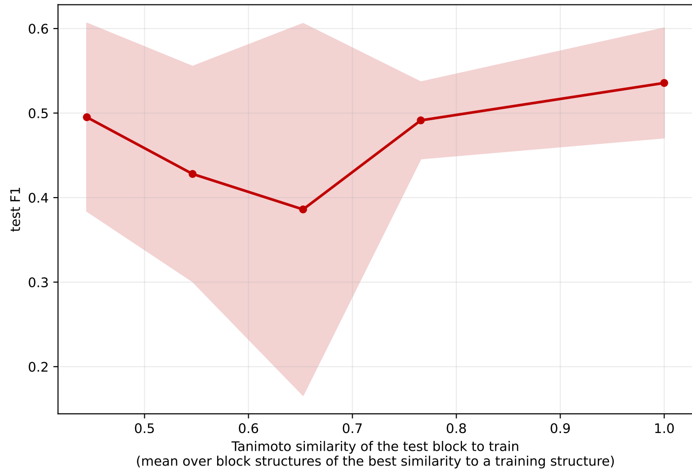
descriptors_head_family_neutral_lipprop_lcs_protbind6 [lipid_coldsplit, random]
