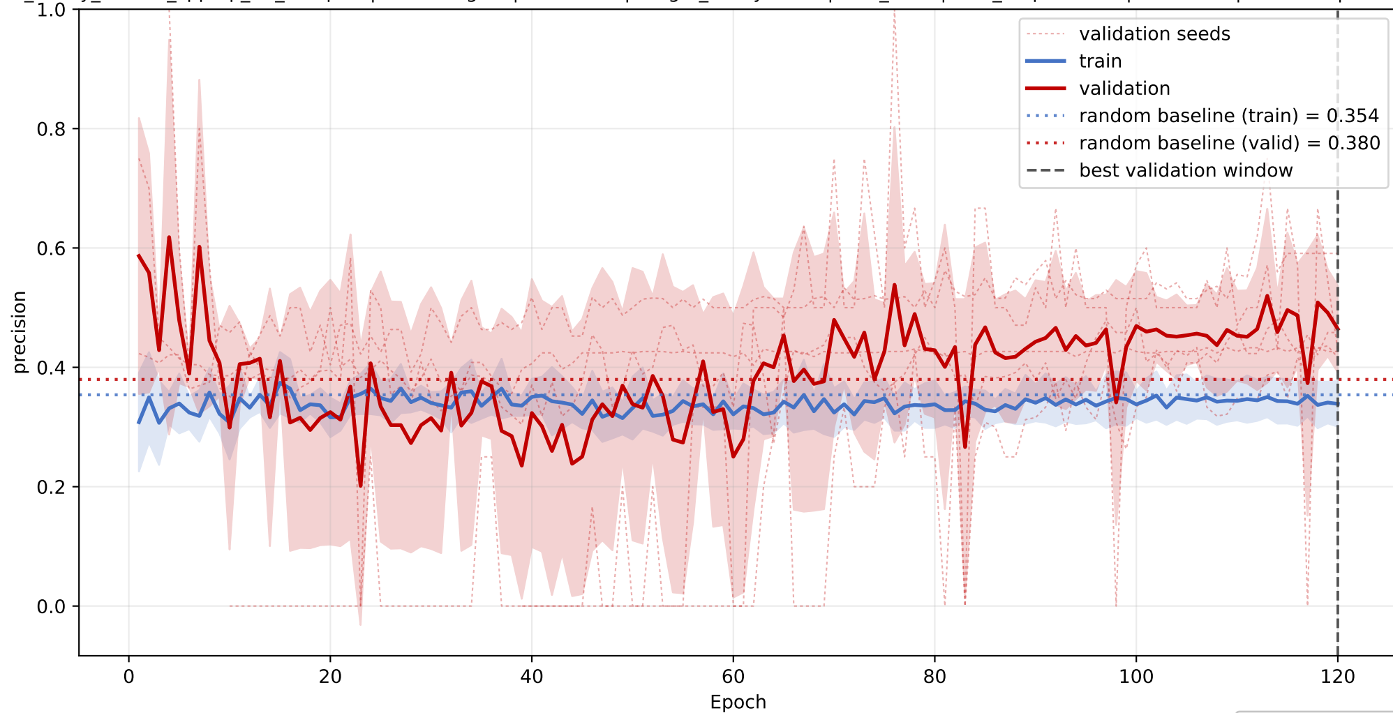
phosphorus_free: mean precision learning curve across seeds
