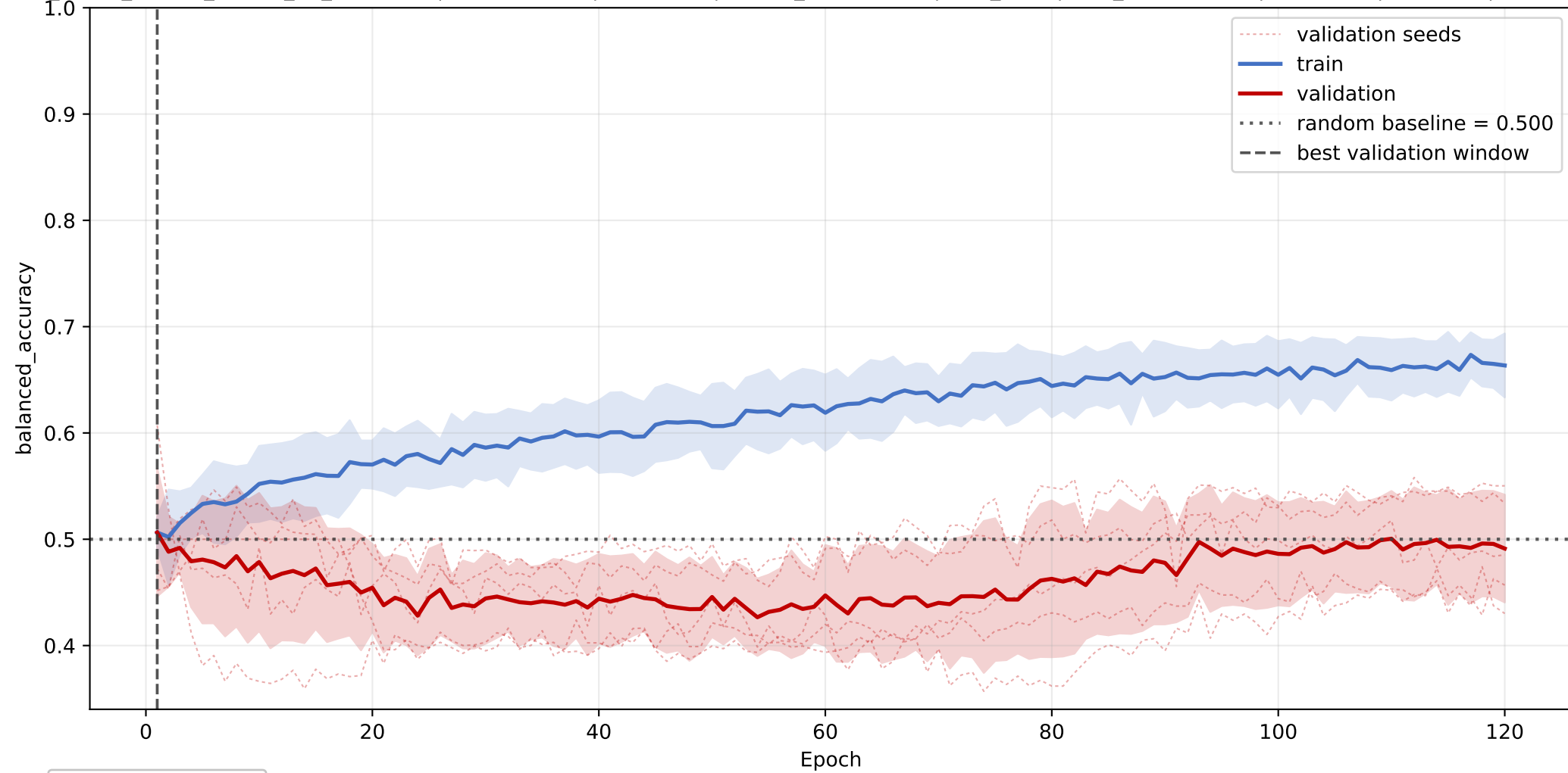
choline: mean balanced_accuracy learning curve across seeds
