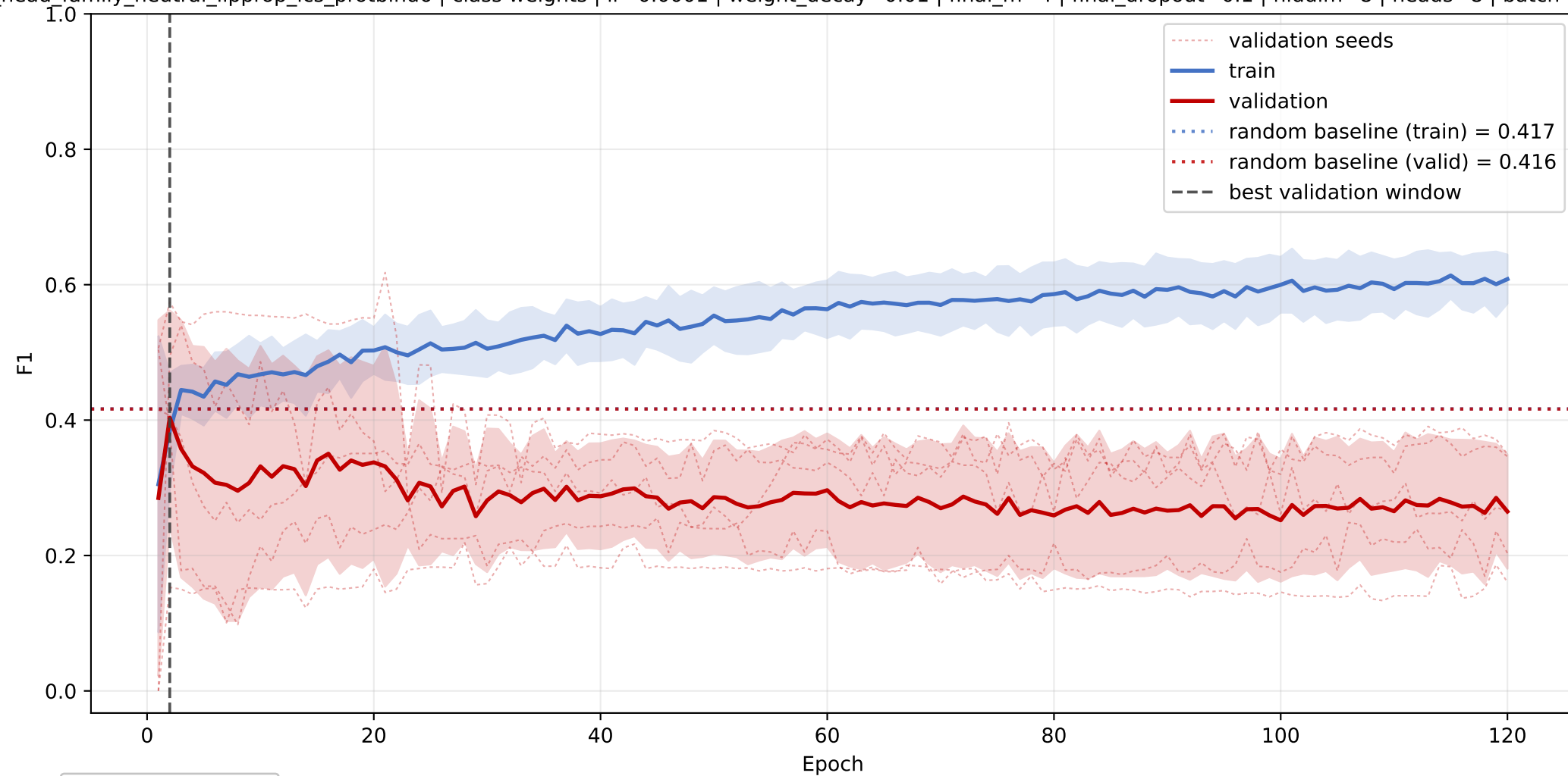
choline: mean F1 learning curve across seeds
