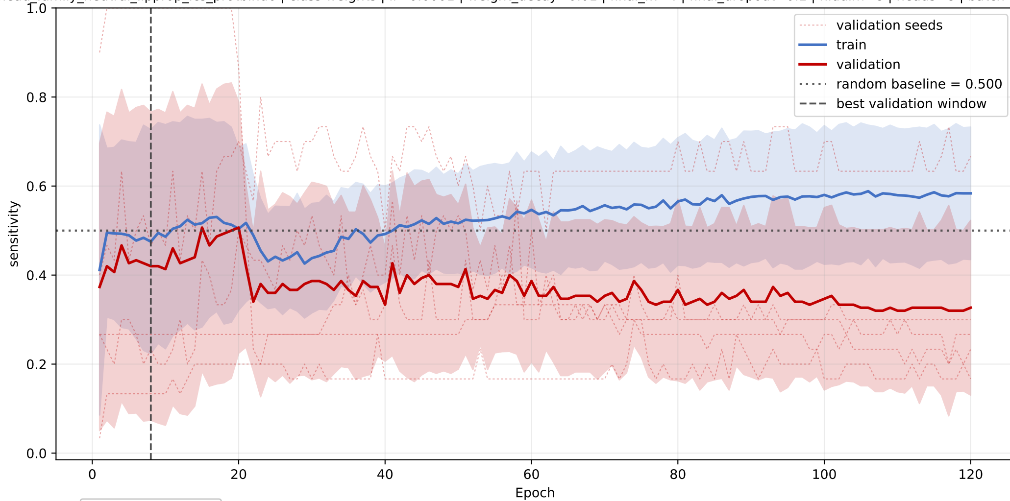
phosphorus_free: mean sensitivity learning curve across seeds
