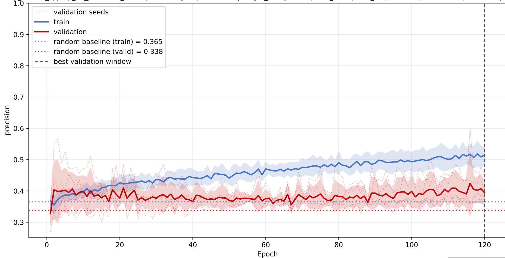
anionic: mean precision learning curve across seeds
