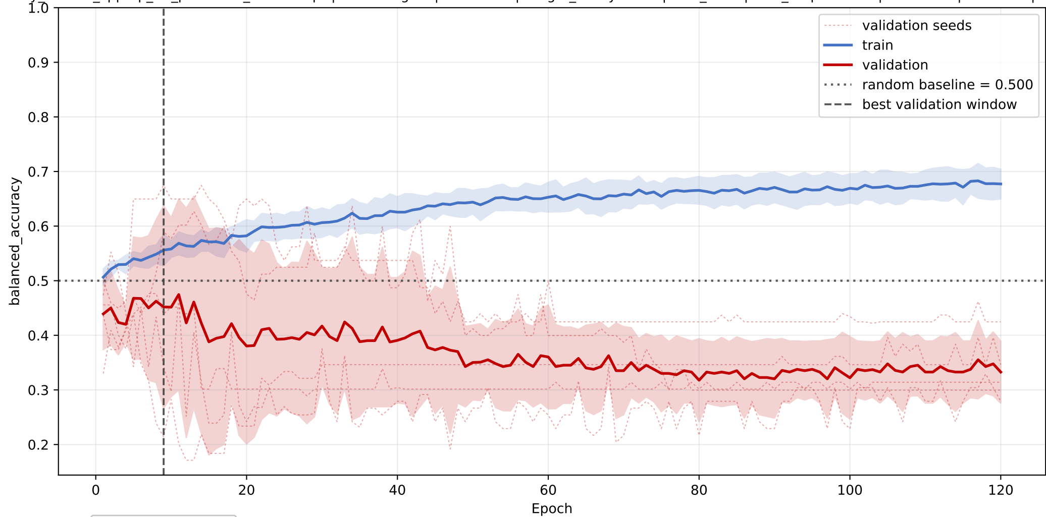
sphingolipids: mean balanced_accuracy learning curve across seeds
