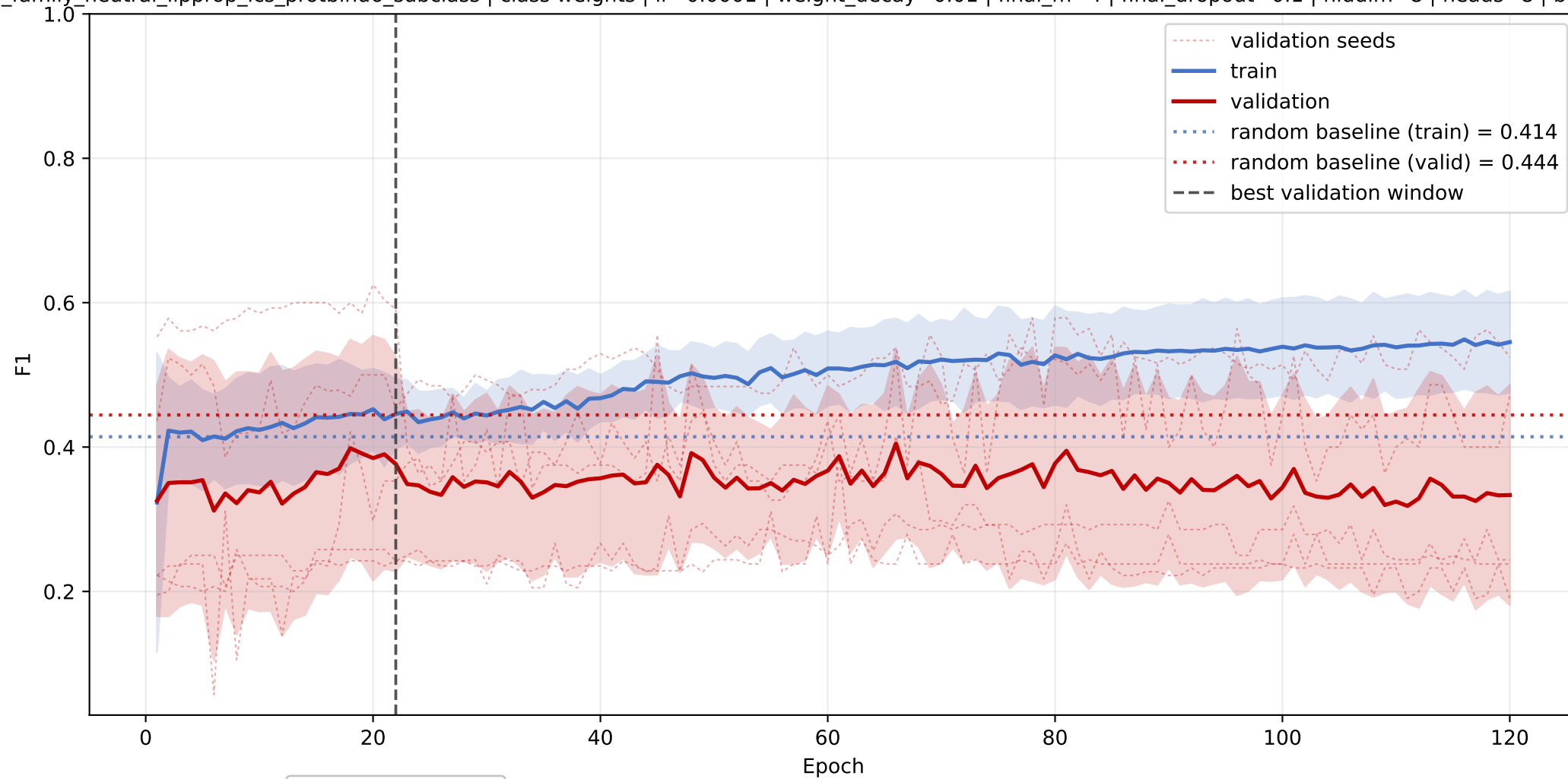
FA: mean F1 learning curve across seeds
