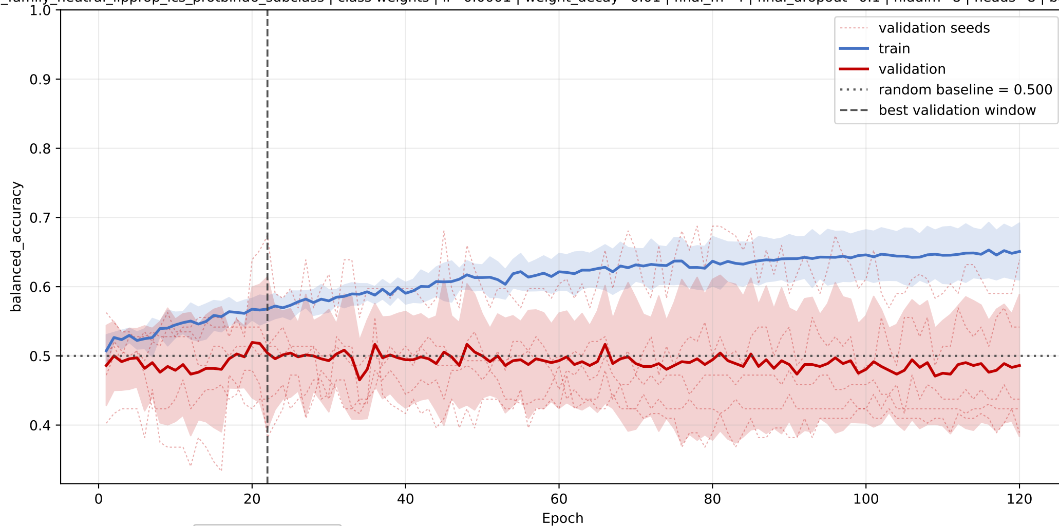
FA: mean balanced_accuracy learning curve across seeds
