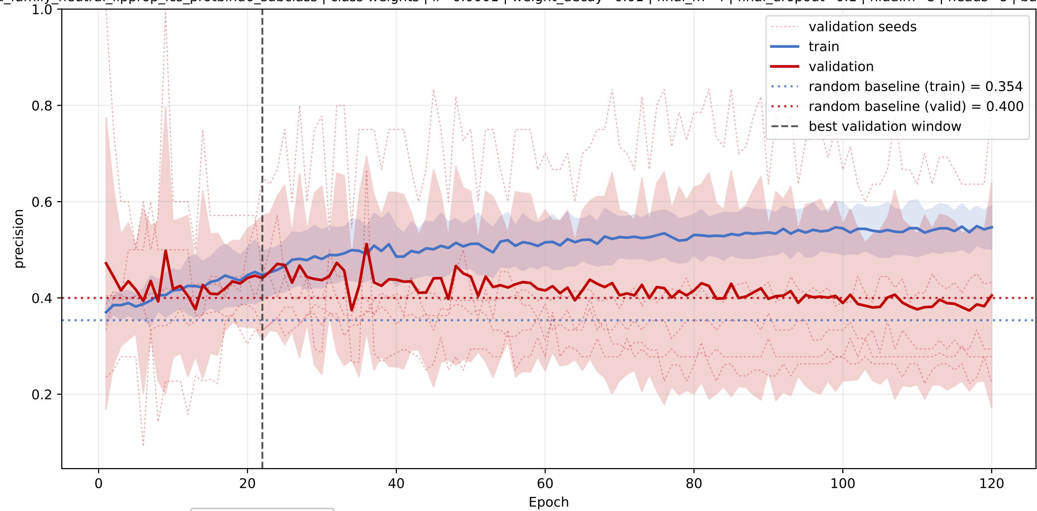
FA: mean precision learning curve across seeds
