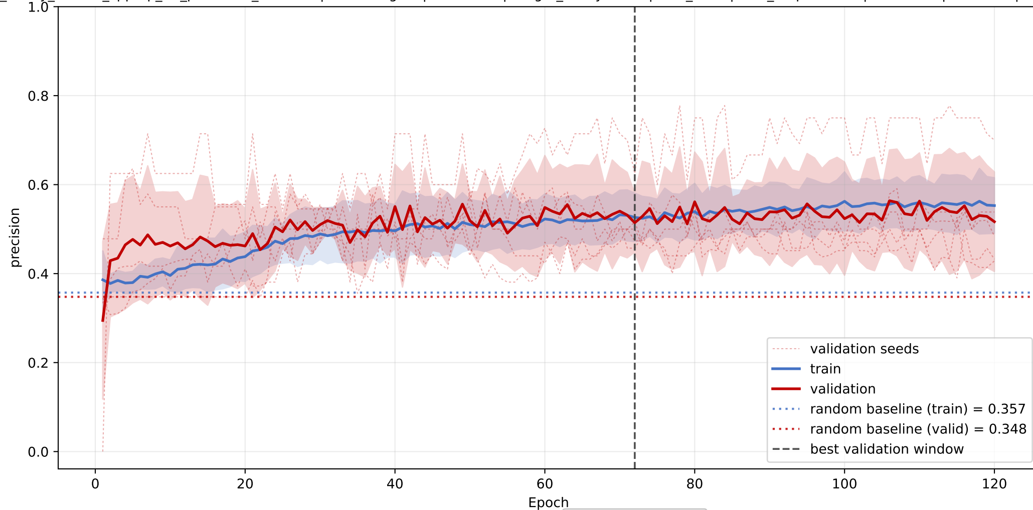
LPC+LPE+LPG: mean precision learning curve across seeds
