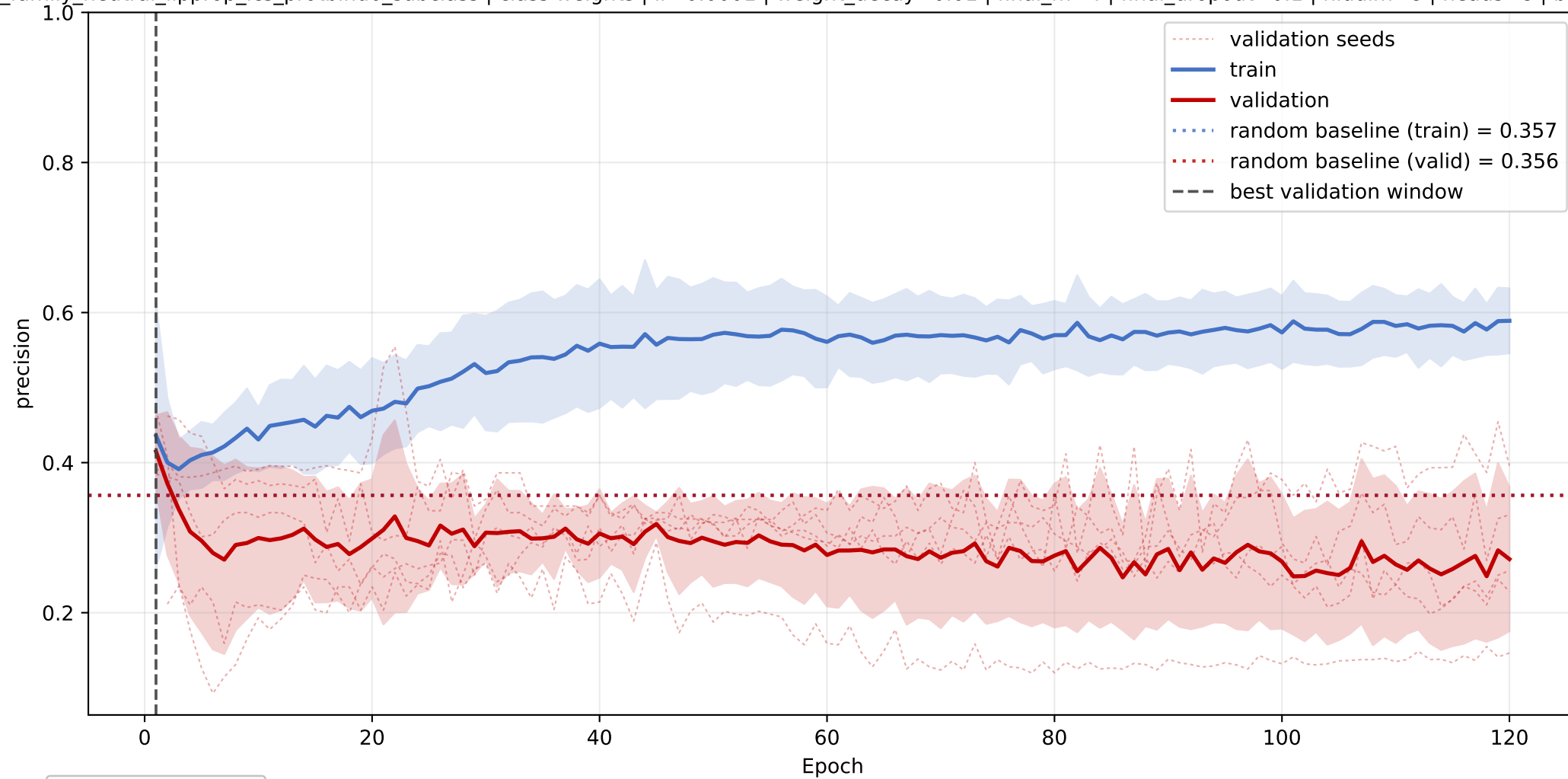
PC: mean precision learning curve across seeds
