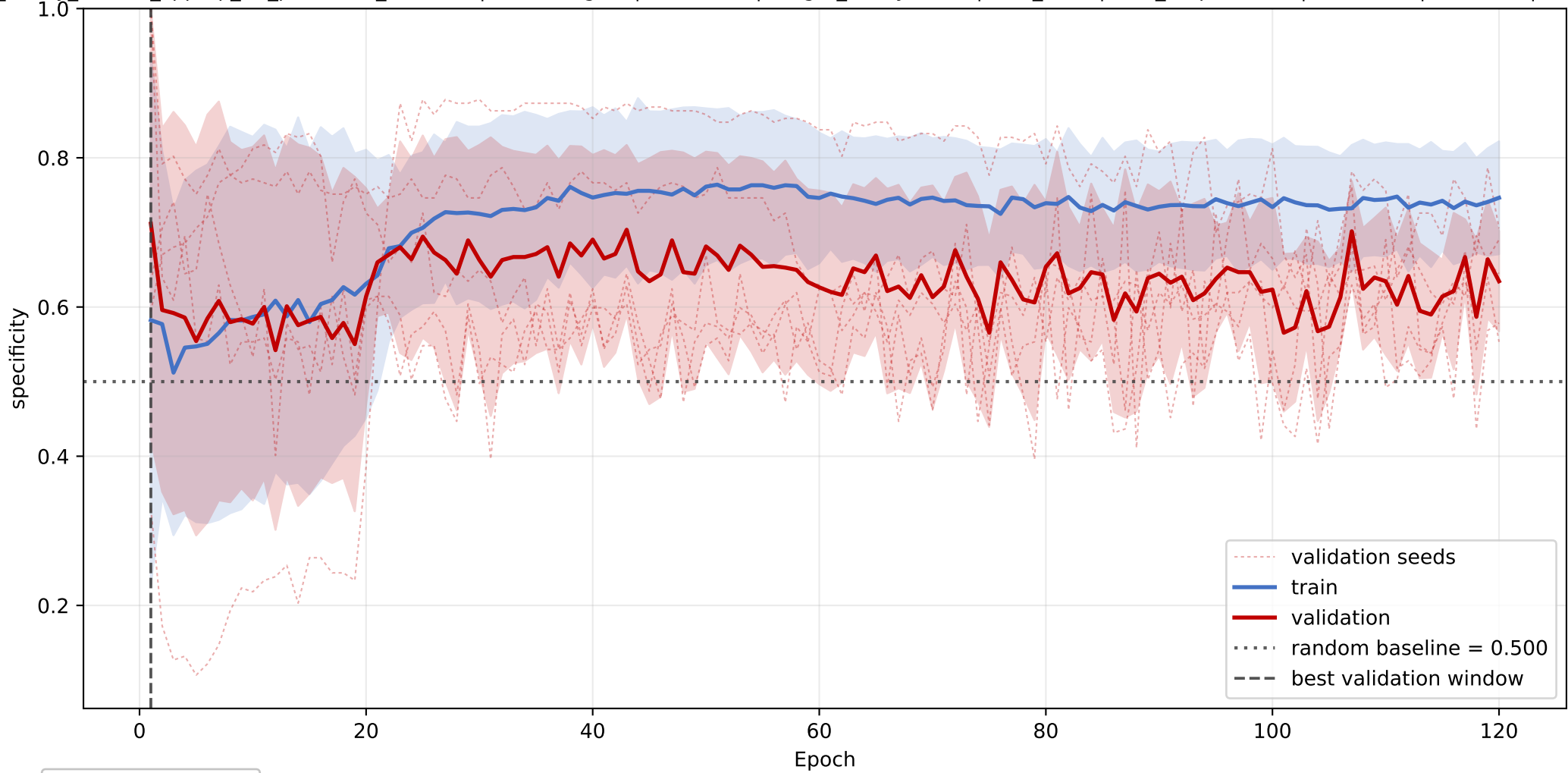
PC: mean specificity learning curve across seeds
