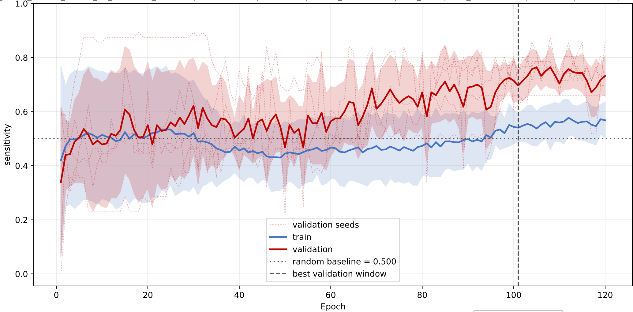
PG: mean sensitivity learning curve across seeds
