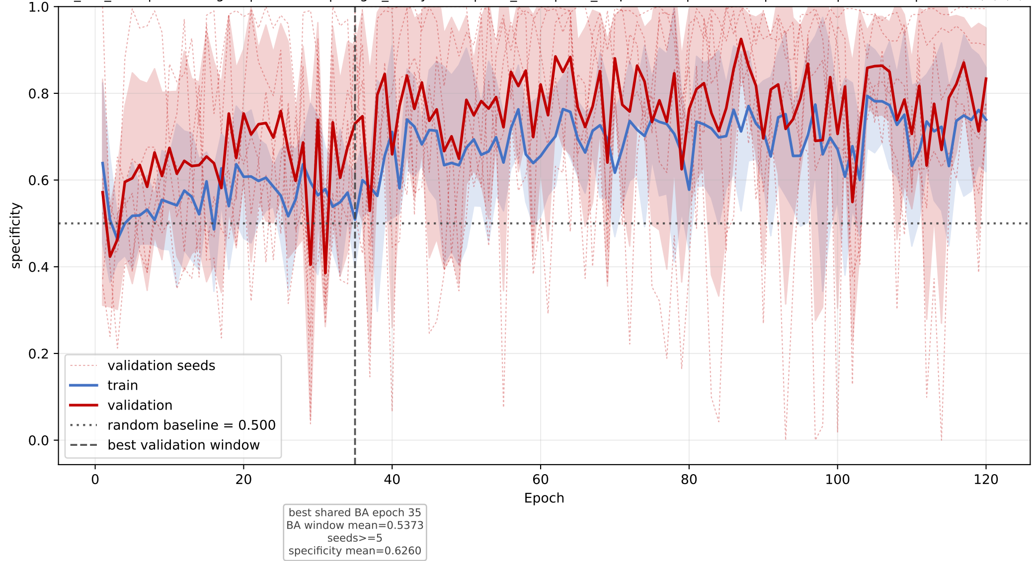
species15: mean specificity learning curve across seeds
