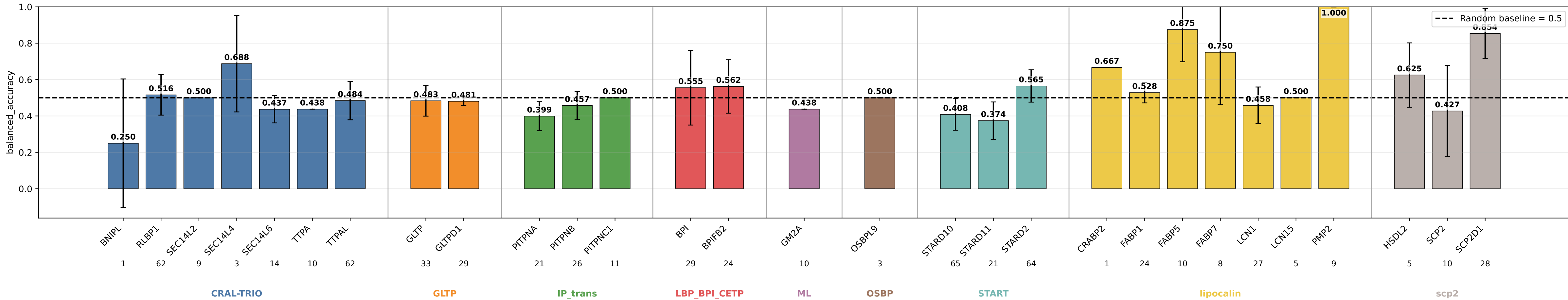
dh_s15_mbw_hid16 balanced_accuracy by subgroup dh_s15_mbw_hid16 | class weights | lr=0.0001 | weight_decay=0.01 | final_m=4 | final_dropout=0.1 | hiddim=16 | heads=8 | batch=16 | ep=120 | seeds=0,1,2,3,4
