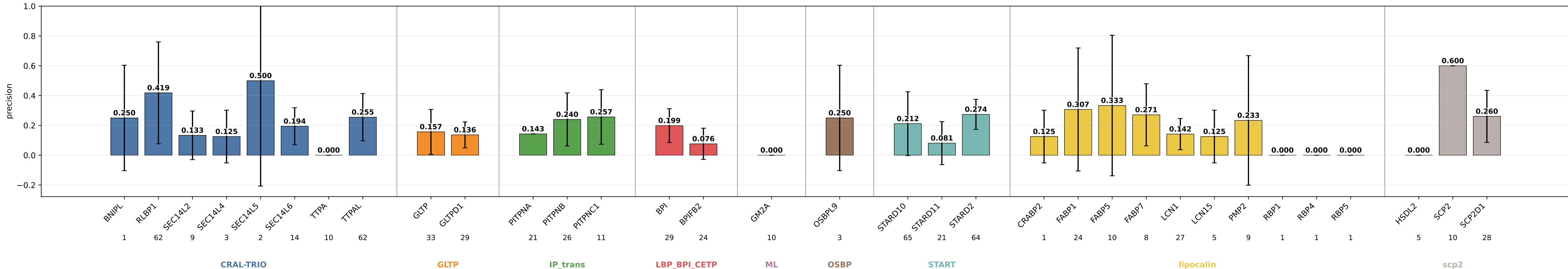
dh_s15_mbw_hid32 precision by subgroup dh_s15_mbw_hid32 | class weights | lr=0.0001 | weight_decay=0.01 | final_m=4 | final_dropout=0.1 | hiddim=32 | heads=8 | batch=16 | ep=120 | seeds=0,1,2,3,4
