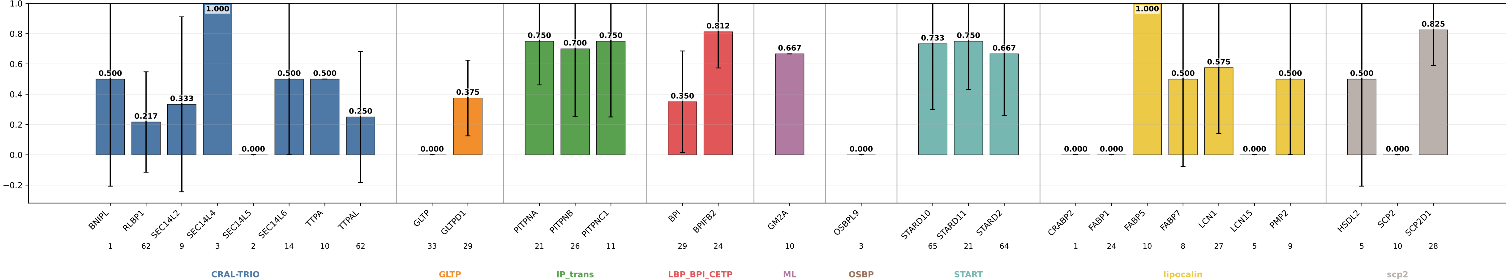
dh_s15_mbw_hid32_d12 sensitivity by subgroup dh_s15_mbw_hid32_d12 | class weights | lr=0.0001 | weight_decay=0.01 | final_m=4 | final_dropout=0.1 | hiddim=32 | heads=8 | batch=16 | ep=120 | seeds=0,1,2,3,4
