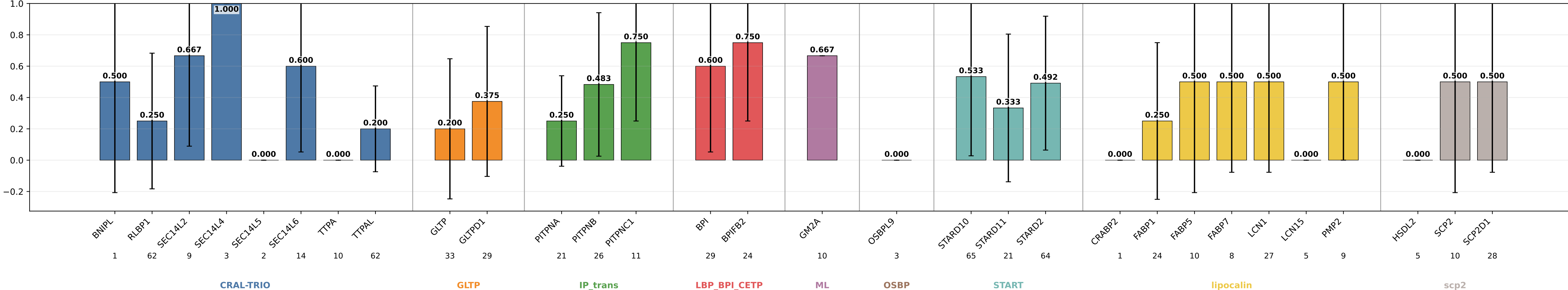
dh_s15_mbw_hid32_d14 sensitivity by subgroup dh_s15_mbw_hid32_d14 | class weights | lr=0.0001 | weight_decay=0.01 | final_m=4 | final_dropout=0.1 | hiddim=32 | heads=8 | batch=16 | ep=120 | seeds=0,1,2,3,4
