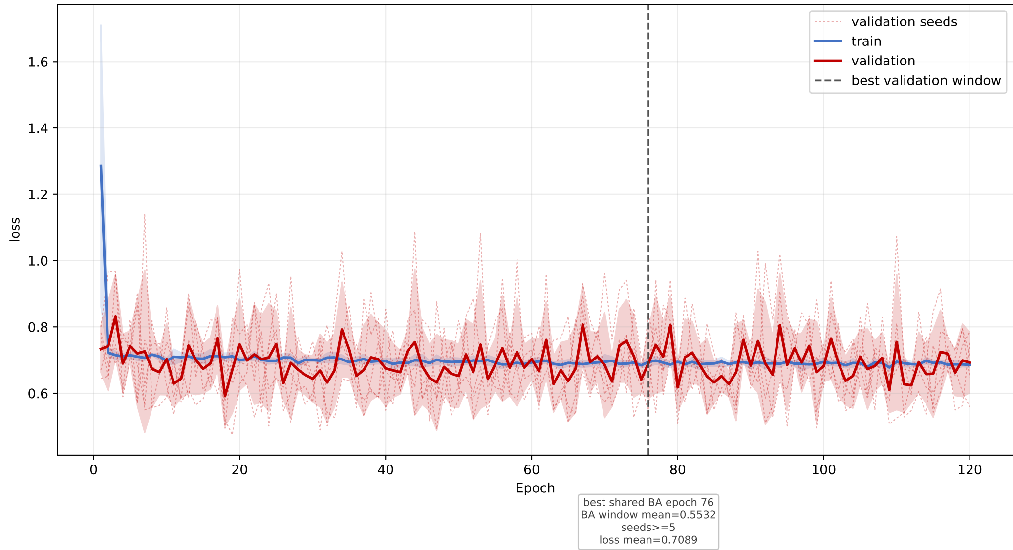
species15: mean loss learning curve across seeds
