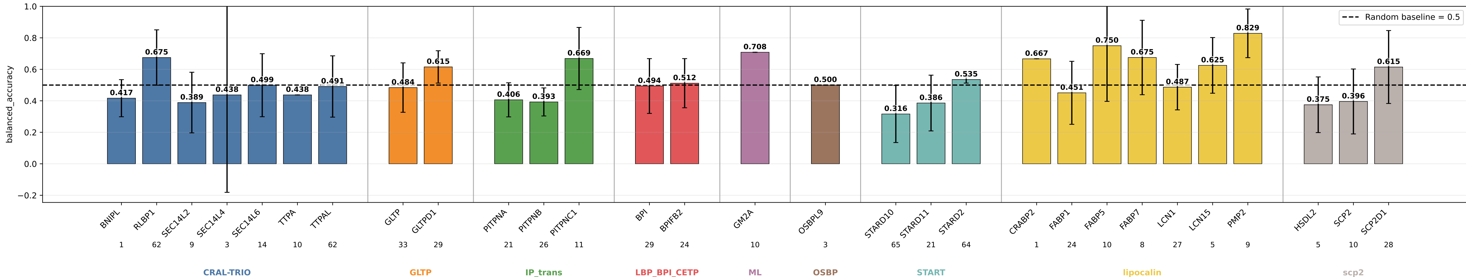
dh_s15_mbw_hid32_lr3e4 balanced_accuracy by subgroup dh_s15_mbw_hid32_lr3e4 | class weights | lr=0.0003 | weight_decay=0.01 | final_m=4 | final_dropout=0.1 | hiddim=32 | heads=8 | batch=16 | ep=120 | seeds=0,1,2,3,4
