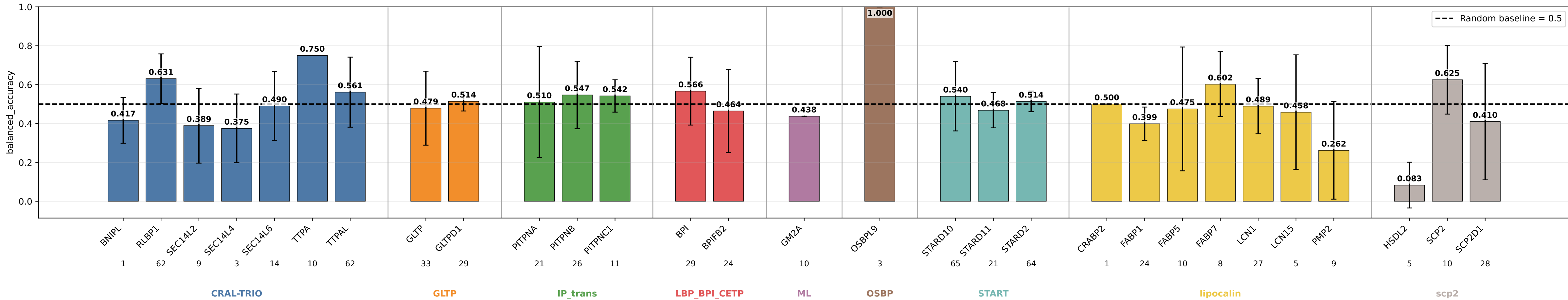
dh_s15_mbw_hid32_m8 balanced_accuracy by subgroup dh_s15_mbw_hid32_m8 | class weights | lr=0.0001 | weight_decay=0.01 | final_m=4 | final_dropout=0.1 | hiddim=32 | heads=8 | batch=16 | ep=120 | seeds=0,1,2,3,4
