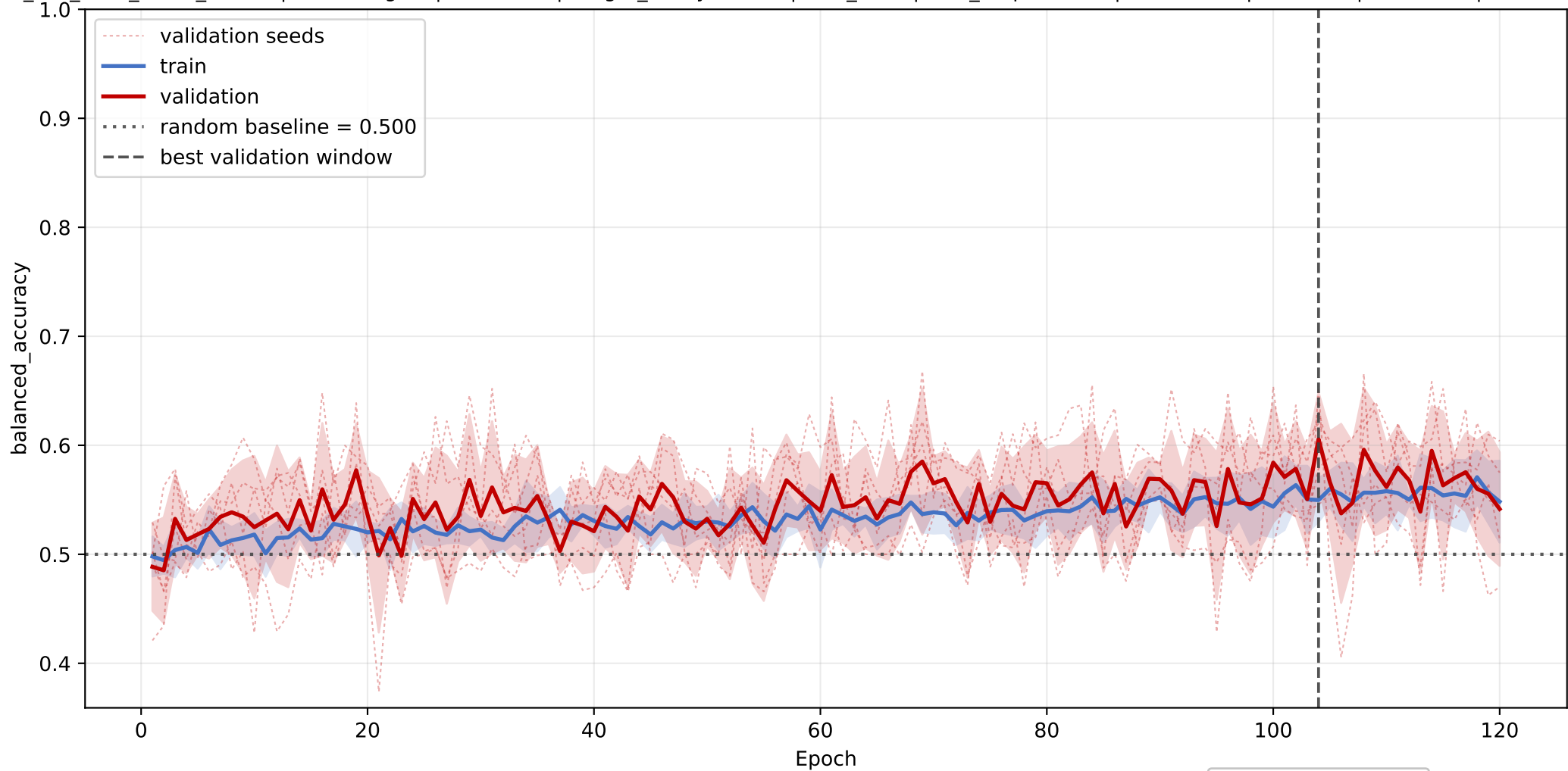
species15: mean balanced_accuracy learning curve across seeds
