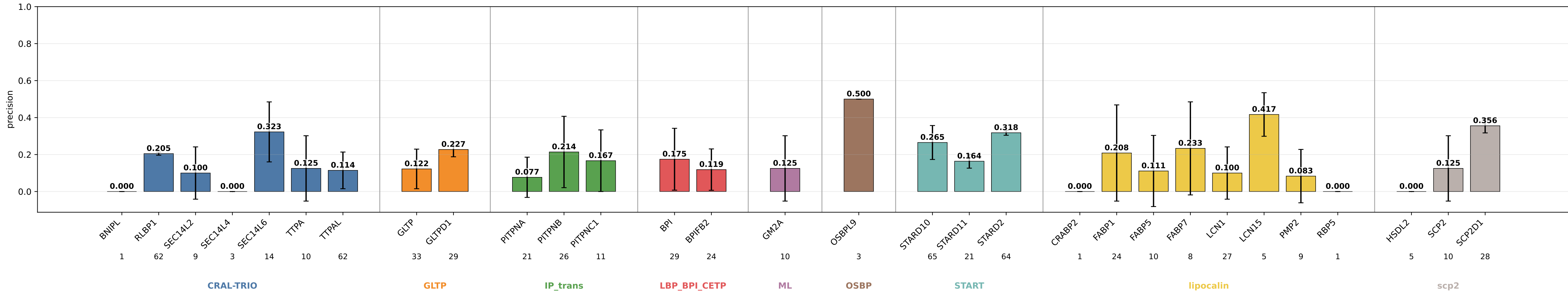
dh_s15_mbw_hid64 precision by subgroup dh_s15_mbw_hid64 | class weights | lr=0.0001 | weight_decay=0.01 | final_m=4 | final_dropout=0.1 | hiddim=64 | heads=8 | batch=16 | ep=120 | seeds=0,1,2,3,4
