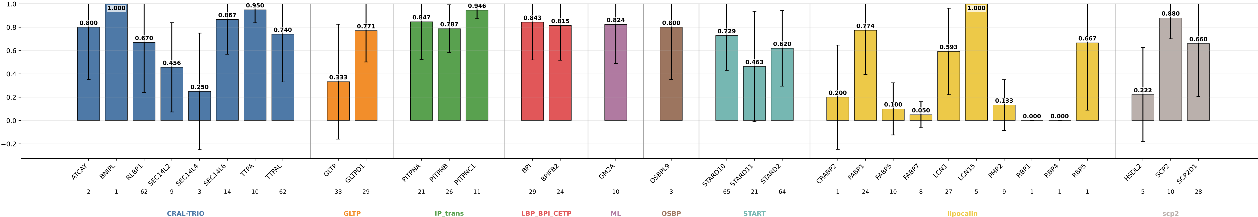
geometric_edge_mlp_protgeom_family_neutral_normalized_bilinear_fusion_bilinear_norm_lcs_balanced_lipid_classes_advprot_protfull sensitivity by subgroup geometric_edge_mlp_protgeom_family_neutral_normalized_bilinear_fusion_bilinear_norm_lcs_balanced_lipid_classes_advprot_protfull | class weights | lr=0.0001 | weight_decay=0.01 | final_m=4 | final_dropout=0.1 | hiddim=8 | heads=8 | batch=16 | ep=120 | seeds=0,1,2,3,4
