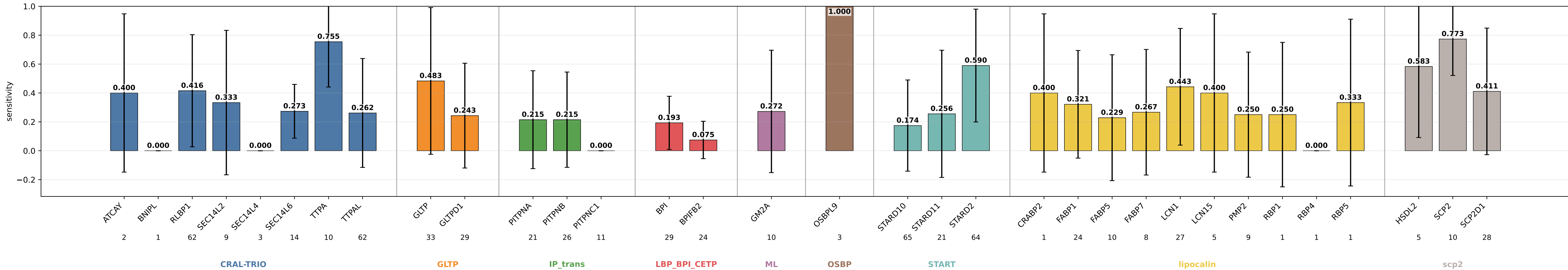
geometric_edge_mlp_protgeom_family_neutral_normalized_bilinear_fusion_bilinear_norm_lcs_esm3_protunion14 sensitivity by subgroup geometric_edge_mlp_protgeom_family_neutral_normalized_bilinear_fusion_bilinear_norm_lcs_esm3_protunion14 | class weights | lr=0.0001 | weight_decay=0.01 | final_m=4 | final_dropout=0.1 | hiddim=8 | heads=8 | batch=16 | ep=120 | seeds=0,1,2,3,4
