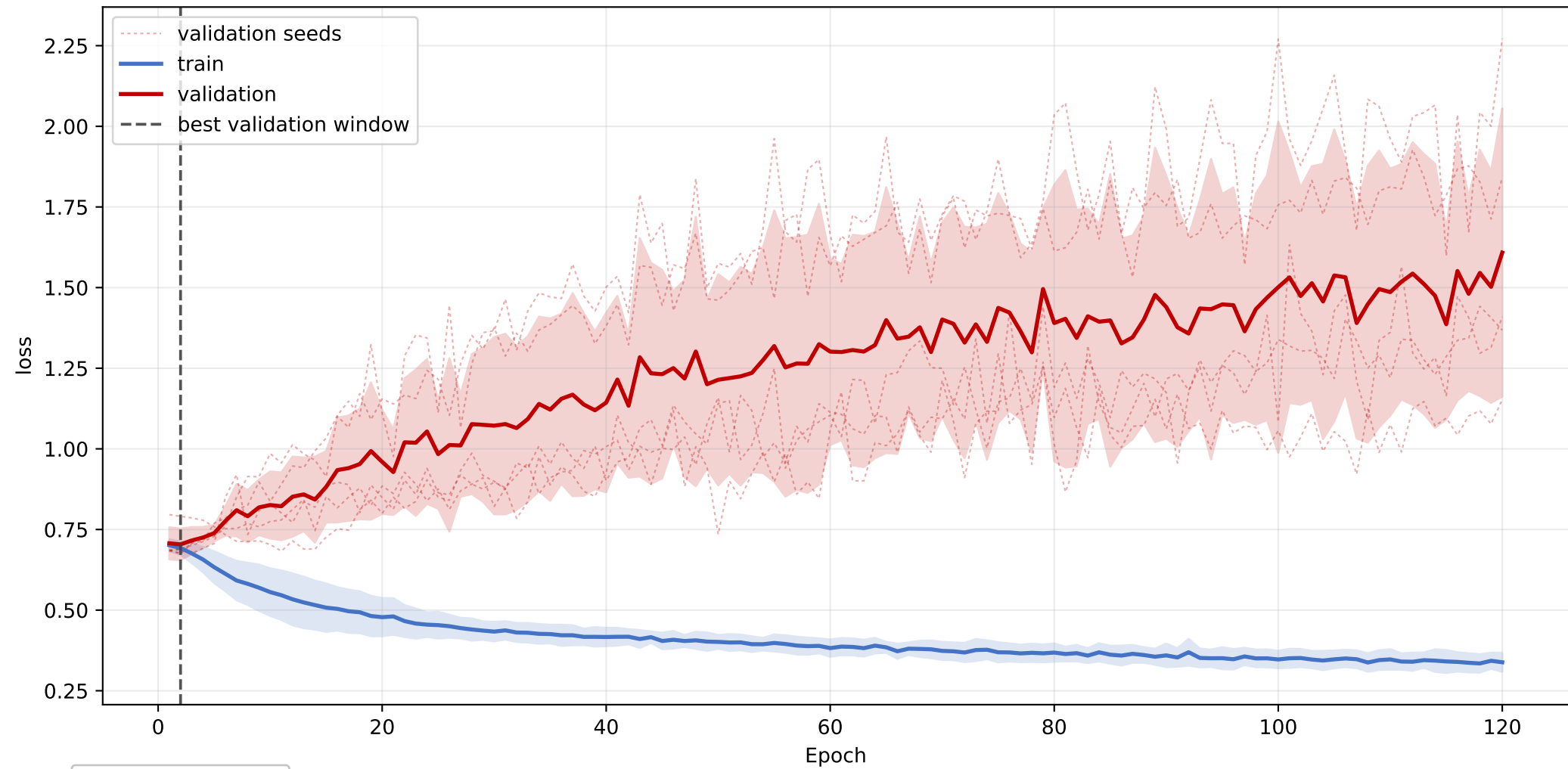
sphingolipids: mean loss learning curve across seeds
