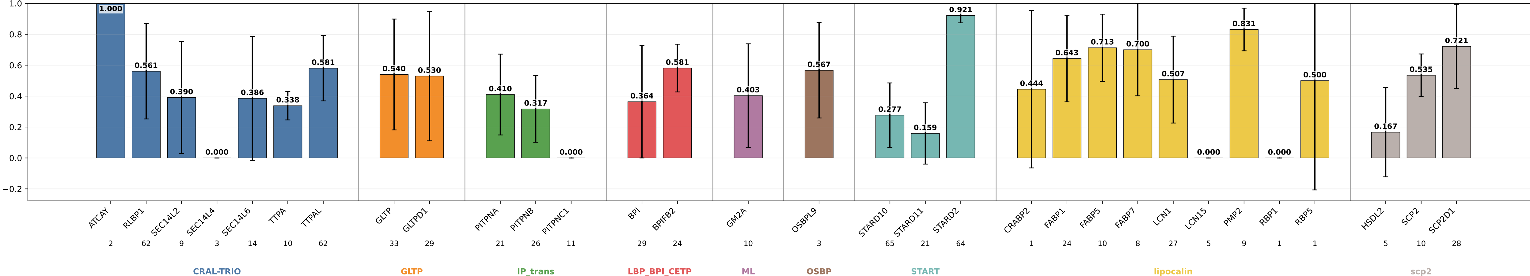
geometric_edge_mlp_protgeom_family_neutral_normalized_bilinear_fusion_bilinear_norm_lcs_esm3_protunion14_prothid32 precision by subgroup geometric_edge_mlp_protgeom_family_neutral_normalized_bilinear_fusion_bilinear_norm_lcs_esm3_protunion14_prothid32 | class weights | lr=0.0001 | weight_decay=0.01 | final_m=4 | final_dropout=0.1 | hiddim=8 | heads=8 | batch=16 | ep=120 | seeds=0,1,2,3,4
