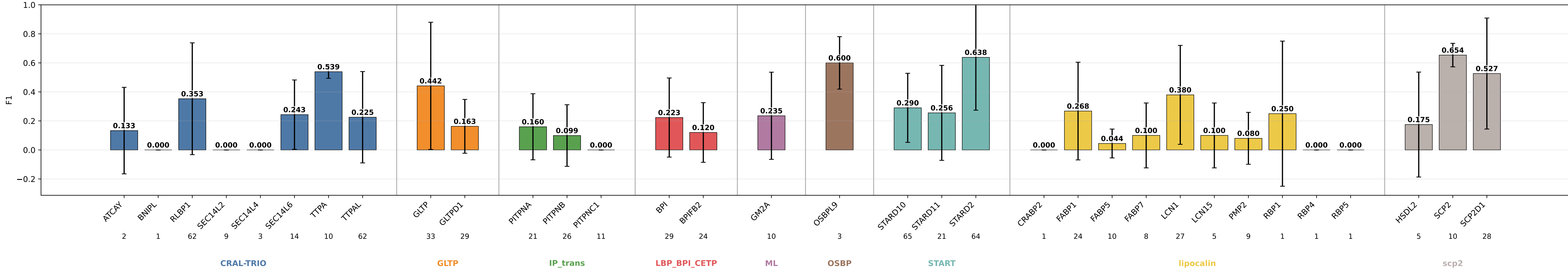
geometric_edge_mlp_protgeom_family_neutral_normalized_bilinear_fusion_bilinear_norm_lcs_esm3_protunion14_prothid32_pocketchem4 F1 by subgroup geometric_edge_mlp_protgeom_family_neutral_normalized_bilinear_fusion_bilinear_norm_lcs_esm3_protunion14_prothid32_pocketchem4 | class weights | lr=0.0001 | weight_decay=0.01 | final_m=4 | final_dropout=0.1 | hiddim=8 | heads=8 | batch=16 | ep=120 | seeds=0,1,2,3,4
