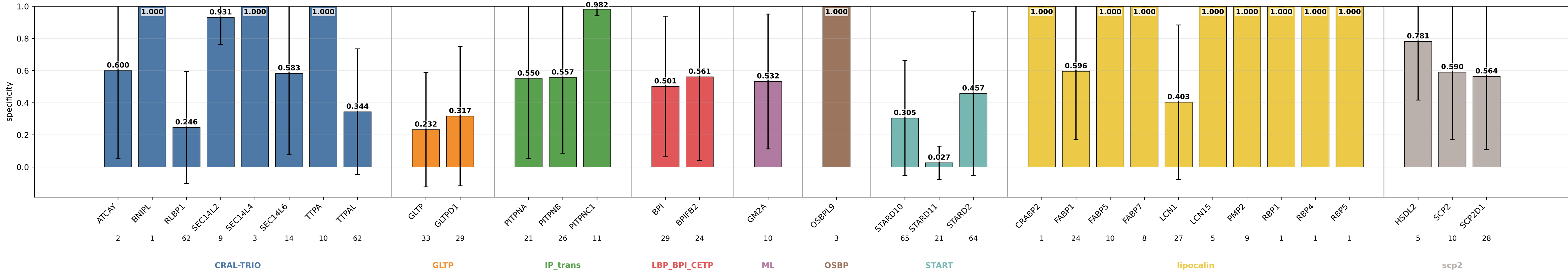
geometric_edge_mlp_protgeom_family_neutral_normalized_bilinear_fusion_bilinear_norm_lcs_esm3_protunion14_prothid32_rotneg specificity by subgroup geometric_edge_mlp_protgeom_family_neutral_normalized_bilinear_fusion_bilinear_norm_lcs_esm3_protunion14_prothid32_rotneg | class weights | lr=0.0001 | weight_decay=0.01 | final_m=4 | final_dropout=0.1 | hiddim=8 | heads=8 | batch=16 | ep=120 | seeds=0,1,2,3,4
