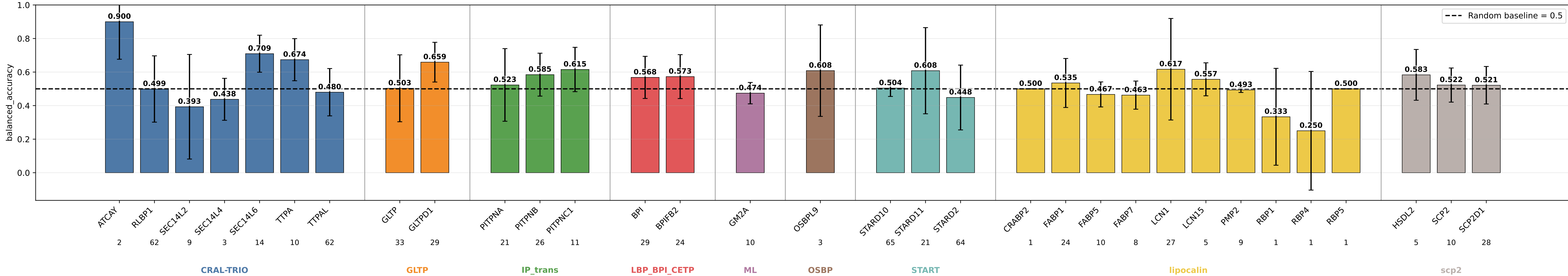
geometric_edge_mlp_protgeom_family_neutral_normalized_bilinear_fusion_bilinear_norm_lcs_protbind6_prothid16 balanced_accuracy by subgroup geometric_edge_mlp_protgeom_family_neutral_normalized_bilinear_fusion_bilinear_norm_lcs_protbind6_prothid16 | class weights | lr=0.0001 | weight_decay=0.01 | final_m=4 | final_dropout=0.1 | hiddim=8 | heads=8 | batch=16 | ep=120 | seeds=0,1,2,3,4
