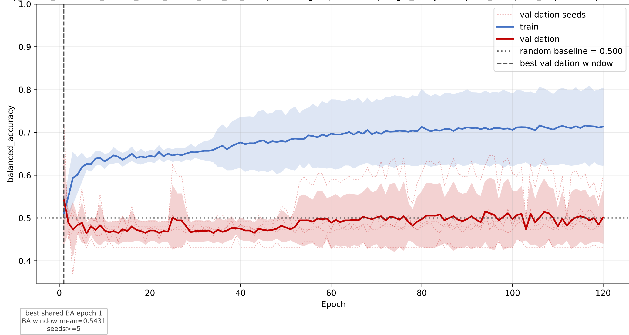
lipocalin: mean balanced_accuracy learning curve across seeds
