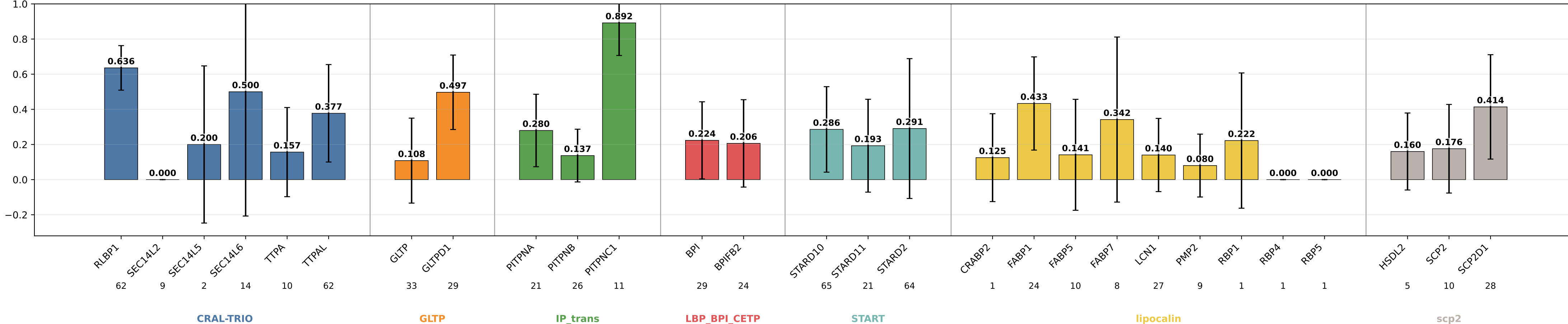
geometric_edge_mlp_protgeom_family_neutral_normalized_bilinear_fusion_bilinear_norm_rim_ev28 F1 by subgroup geometric_edge_mlp_protgeom_family_neutral_normalized_bilinear_fusion_bilinear_norm_rim_ev28 | class weights | lr=0.0001 | weight_decay=0.01 | final_m=4 | final_dropout=0.1 | hiddim=8 | heads=8 | batch=16 | ep=120 | seeds=0,1,2,3,4
