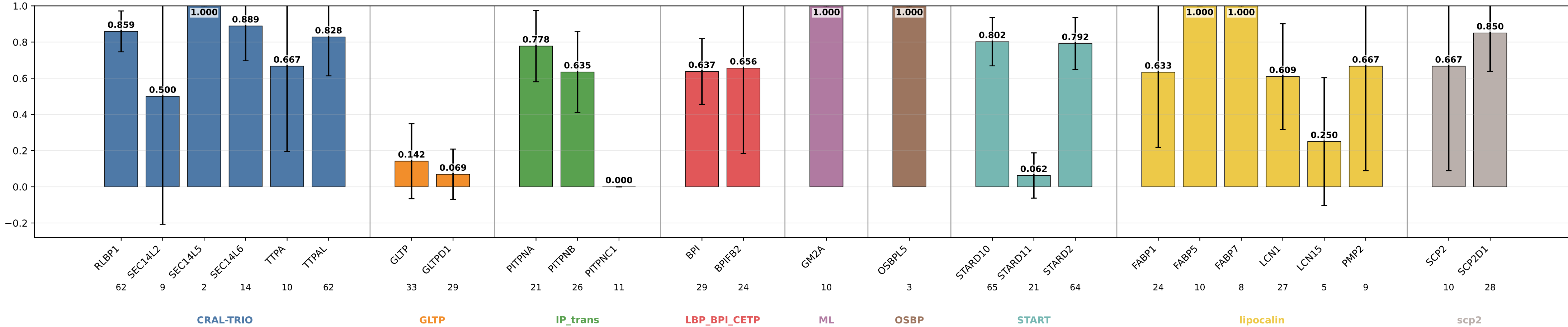
geometric_edge_mlp_protgeom_family_neutral_normalized_bilinear_fusion_bilinear_norm_rim_ev28_rand AUC by subgroup geometric_edge_mlp_protgeom_family_neutral_normalized_bilinear_fusion_bilinear_norm_rim_ev28_rand | class weights | lr=0.0001 | weight_decay=0.01 | final_m=4 | final_dropout=0.1 | hiddim=8 | heads=8 | batch=16 | ep=120 | seeds=0,1,2,3,4
