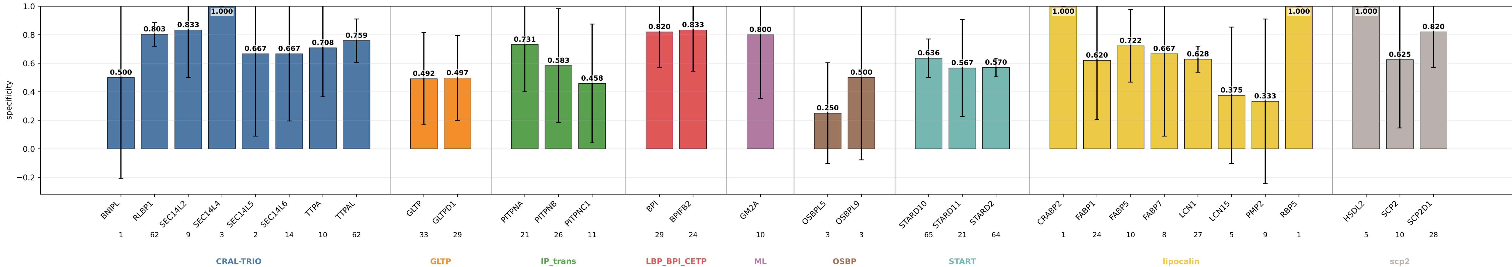
geometric_edge_mlp_protgeom_family_neutral_normalized_bilinear_fusion_bilinear_norm_rim_ev28_rand specificity by subgroup geometric_edge_mlp_protgeom_family_neutral_normalized_bilinear_fusion_bilinear_norm_rim_ev28_rand | class weights | lr=0.0001 | weight_decay=0.01 | final_m=4 | final_dropout=0.1 | hiddim=8 | heads=8 | batch=16 | ep=120 | seeds=0,1,2,3,4
