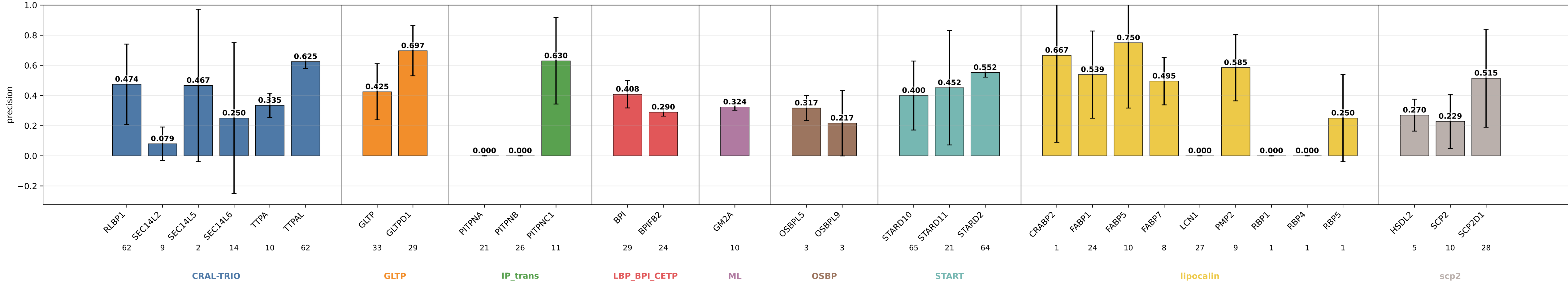
geometric_edge_mlp_protgeom_family_neutral_normalized_bilinear_fusion_bilinear_norm_rim_ev28_rotneg precision by subgroup geometric_edge_mlp_protgeom_family_neutral_normalized_bilinear_fusion_bilinear_norm_rim_ev28_rotneg | class weights | lr=0.0001 | weight_decay=0.01 | final_m=4 | final_dropout=0.1 | hiddim=8 | heads=8 | batch=16 | ep=120 | seeds=0,1,2,3,4
