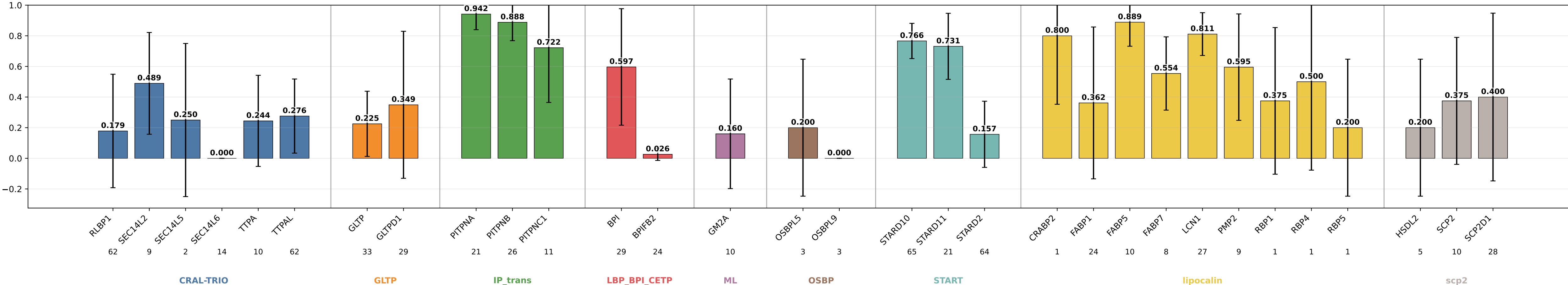
geometric_edge_mlp_protgeom_family_neutral_normalized_bilinear_fusion_bilinear_norm_rim_ev28_rotneg specificity by subgroup geometric_edge_mlp_protgeom_family_neutral_normalized_bilinear_fusion_bilinear_norm_rim_ev28_rotneg | class weights | lr=0.0001 | weight_decay=0.01 | final_m=4 | final_dropout=0.1 | hiddim=8 | heads=8 | batch=16 | ep=120 | seeds=0,1,2,3,4
