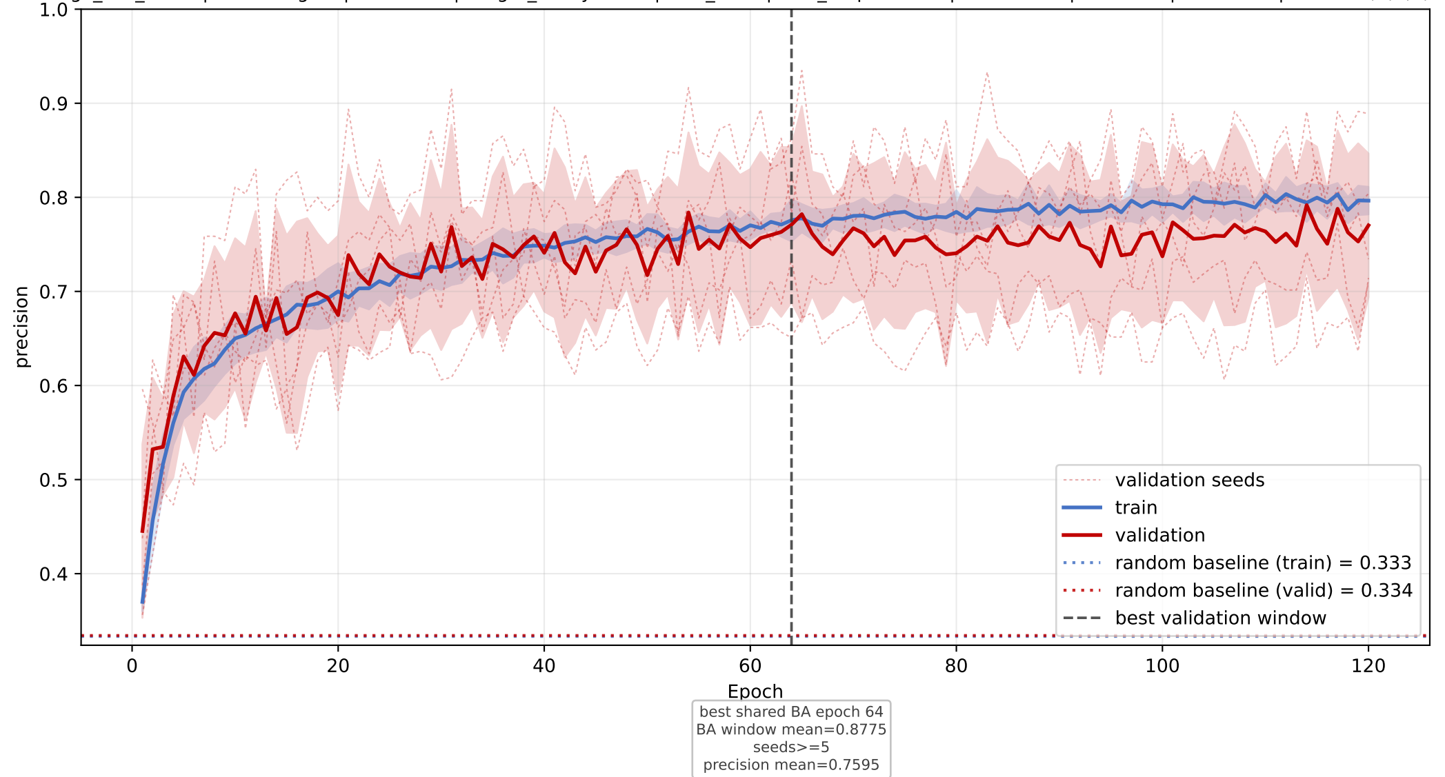
species15: mean precision learning curve across seeds
