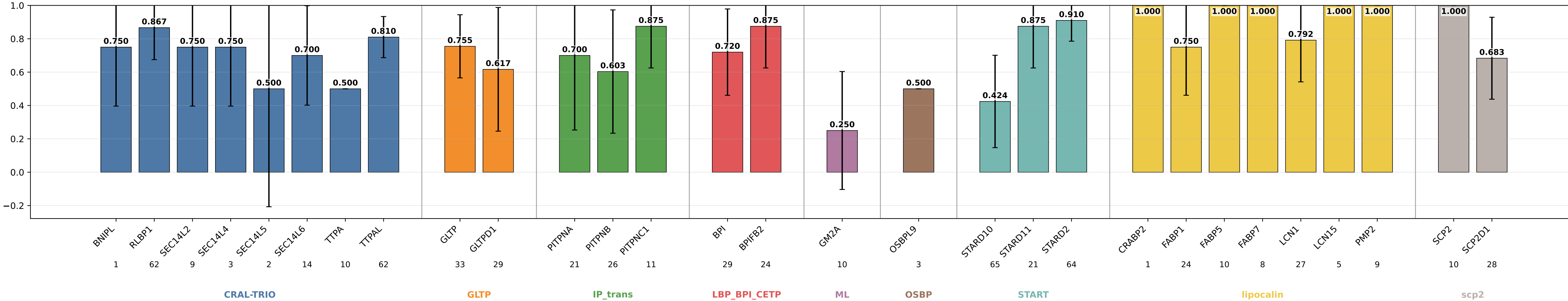
ge_s15_prothid32_dpt0 precision by subgroup ge_s15_prothid32_dpt0 | class weights | lr=0.0001 | weight_decay=0.01 | final_m=4 | final_dropout=0.0 | hiddim=8 | heads=8 | batch=16 | ep=120 | seeds=0,1,2,3,4
