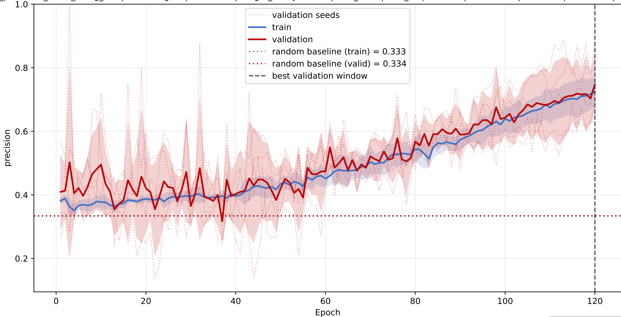
species15: mean precision learning curve across seeds
