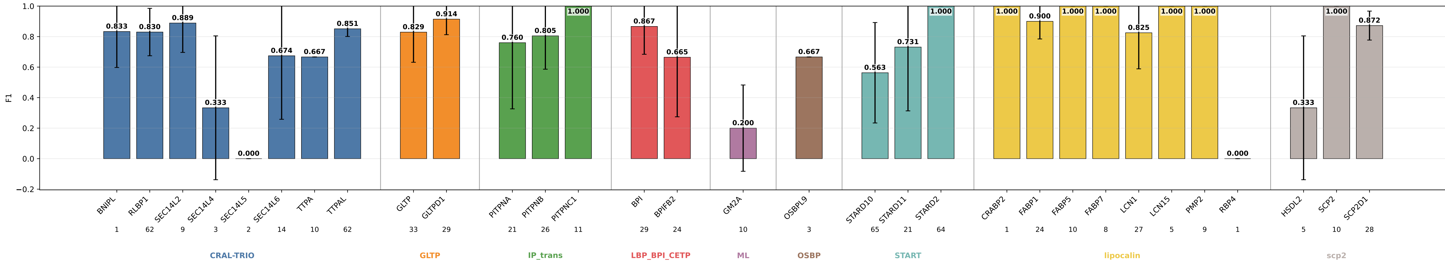
ge_s15_prothid32_hid64_noreg_gnorm F1 by subgroup ge_s15_prothid32_hid64_noreg_gnorm | class weights | lr=0.0001 | weight_decay=1e-05 | final_m=4 | final_dropout=0.0 | hiddim=64 | heads=8 | batch=16 | ep=120 | seeds=0,1,2,3,4
