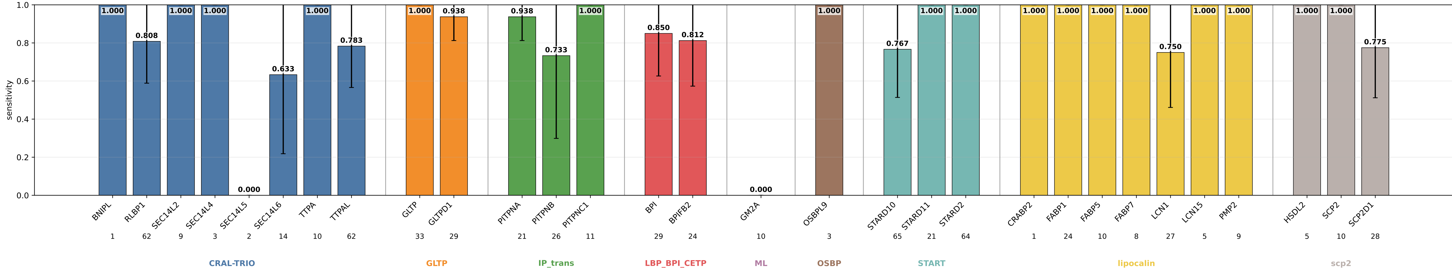
ge_s15_prothid32_hid64_noreg_liphandicap sensitivity by subgroup ge_s15_prothid32_hid64_noreg_liphandicap | class weights | lr=0.0001 | weight_decay=1e-05 | final_m=4 | final_dropout=0.0 | hiddim=64 | heads=8 | batch=16 | ep=120 | seeds=0,1,2,3,4
